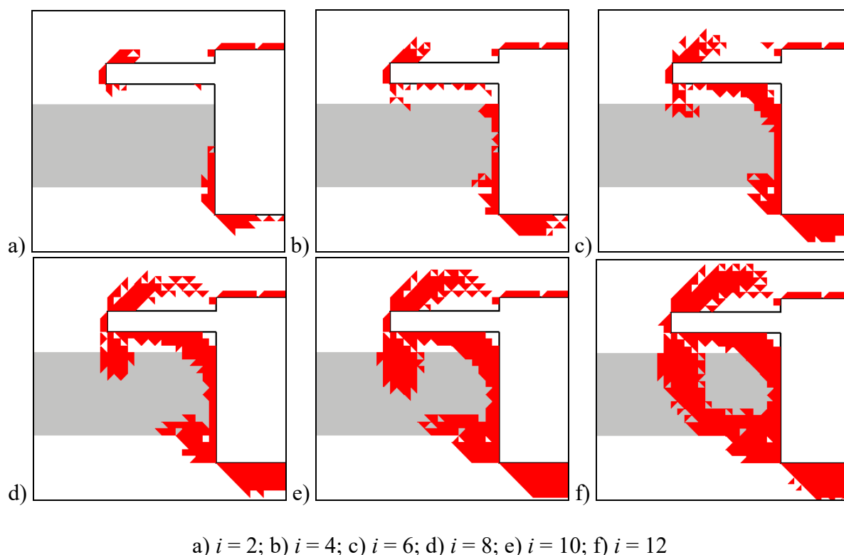
Figure 14 – Temporal progress of the zone of inelastic deformations (red colour) in the mine face with the unloading cavity
