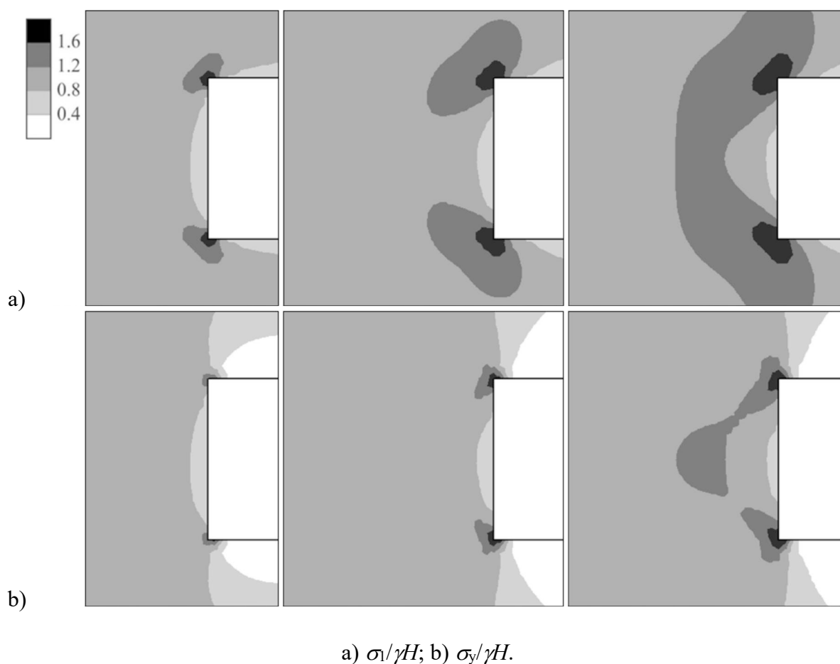
Figure 6 – Distributions of stress parameters values in the moments of time: t = 5 \text{ h} , t = 25 \text{ h} and t = 50 \text{ h}
